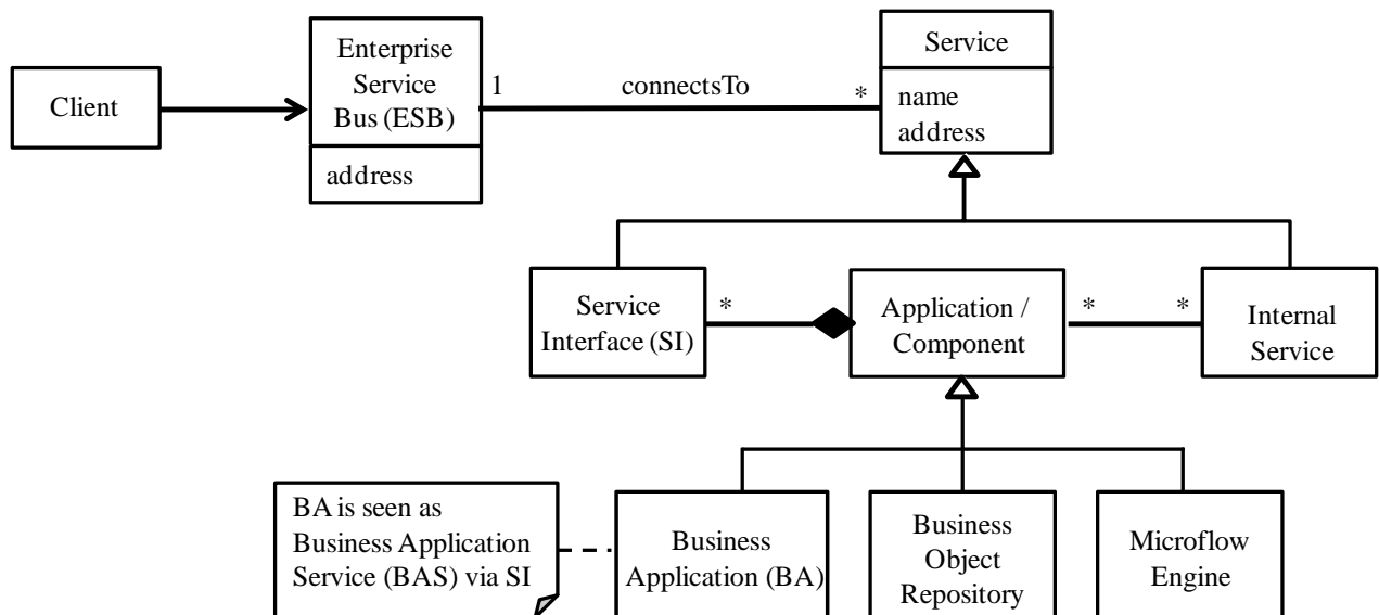
Fig. 1. Enterprise Service Bus (based on [Zdu06])
