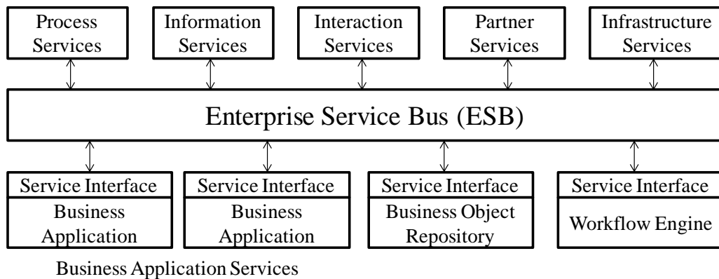
Fig. 1. Enterprise Service Bus (based on [Zdu06])
